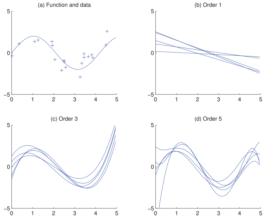
Figure 4.5 (a) Function, f(x) = 2\sin(1.5x) , and one noisy ( \mathcal{N}(0,1) ) dataset sampled from the function. Five samples are taken, each containing twenty instances. (b), (c), (d) are five polynomial fits, namely, g_i(\cdot) , of order 1, 3, and 5. For each case, dotted line is the average of the five fits, namely, \bar{g}(\cdot) .
