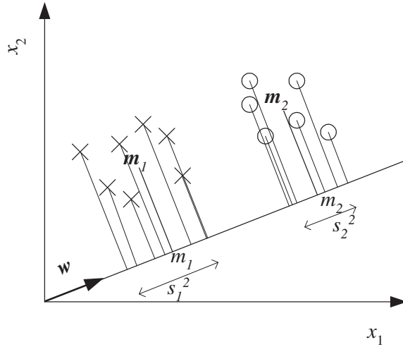
Figure 6.10 Two-dimensional, two-class data projected on \mathbf{w} .
