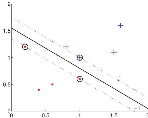
Figure 13.1 For a two-class problem where the instances of the classes are shown by plus signs and dots, the thick line is the boundary and the dashed lines define the margins on either side. Circled instances are the support vectors.
