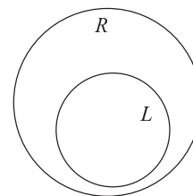
(c) Recall = 1
