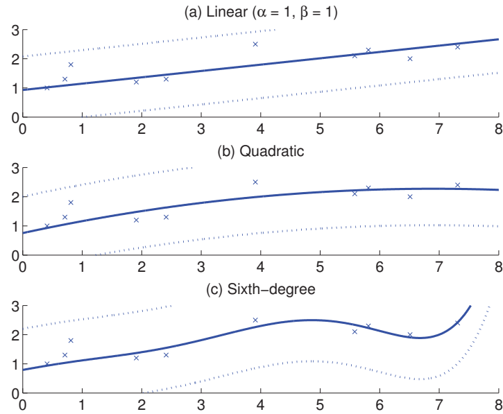
Figure 16.6 Bayesian regression using kernels with one standard deviation error bars: (a) linear: \boldsymbol{\phi}(x) = [1, x]^T , (b) quadratic: \boldsymbol{\phi}(x) = [1, x, x^2]^T , and (c) sixth degree: \boldsymbol{\phi}(x) = [1, x, x^2, x^3, x^4, x^5, x^6]^T .
