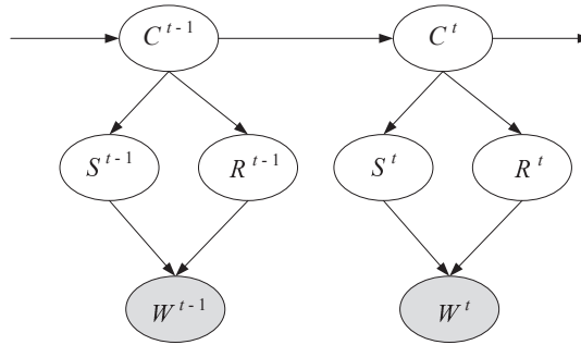
Figure 15.8 A dynamic version where we have a chain of graphs to show dependency in weather on consecutive days.
